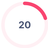
Page Strength
