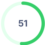
Domain Strength
